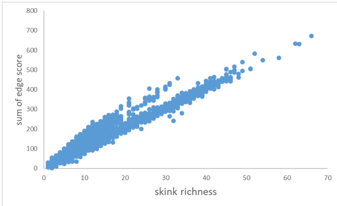
Fig. S2. Distribution of EDGE (Evolutionarily Distinct and Globally Endangered) scores for skinks. (A) Mean of EDGE score within \sim 1^\circ \times 1^\circ degree grid cells, (B) Sum of EDGE score within the same cells. Relationship between mean skink richness and mean EDGE score within cells (C), and skink richness and sum of EDGE score within cells (D).
