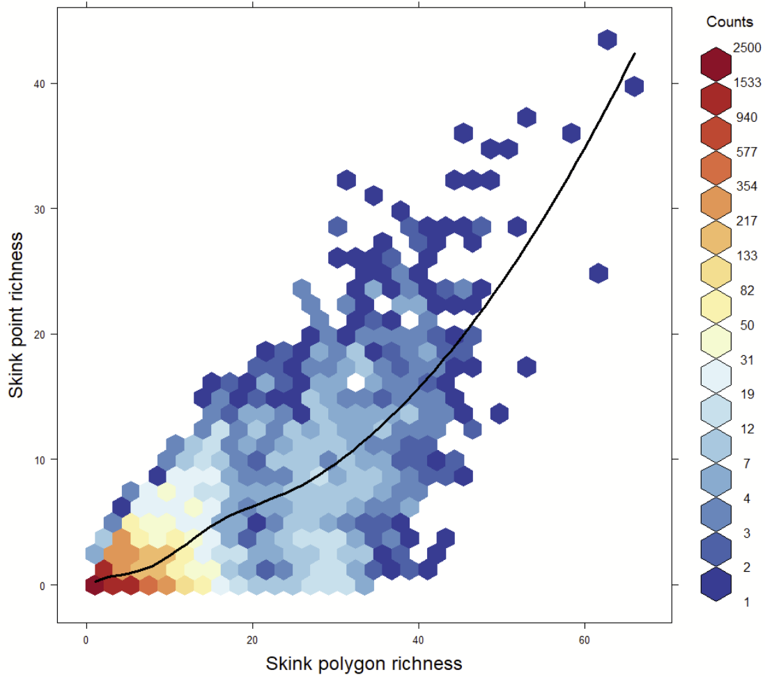
Fig. S1. Comparison of the skink distributional patterns obtained from point locality (A) and polygon (B) data from Global Assessment of Reptile Distributions (GARD; http://www.gardinitiative.org/ ). A hexbin plot (C) indicates that there is a strong relationship between skink richness using both point and polygon data. The black line is a loess fit. Counts refer to the number of observations forming each hexagon, where each observation is a pair of richness values for the same grid cell, one based on point locality data and the other on polygons. Both from GARD ( http://www.gardinitiative.org/ )
