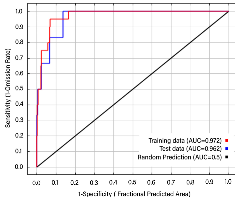
Figure 2. AUC value obtained from ROC analysis to test model predictions.
